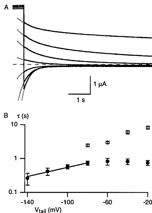
FIGURE 2 Deactivation kinetics of I_{SK} . (A) Tail currents were recorded during repolarization to potentials from -20 to -140 mV, in 20-mV increments, after activation of I_{SK} with a 20-s pulse to 40 mV. Time constants for deactivation were derived by fitting a double exponential to the tail currents (.....). For potentials less than -80 mV, a single exponential was used. (B) Time constants of deactivation plotted on a log scale as a function of tail potential. The data for the fast component of deactivation were fit with a single exponential yielding 2.6e^{V/64} . Bars represent the standard deviation from five experiments.
