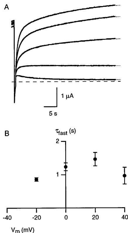
FIGURE 6 Voltage dependence of kinetics of reactivation. ( A ) I_{SK} was activated by a 20-s pulse to 40 mV from a holding potential of -80 mV. The membrane was briefly repolarized (500 ms) to -140 mV to close a fraction of the channels ( \sim 73\% of the tail current deactivated) before reactivation to test potentials between -40 and 40 mV. ( B ) The voltage dependence of reactivation was examined by fitting the rising phase of reactivation with a double exponential, and the fast time constant, \tau_{fast} , was plotted as a function of the test potential. Data represent the mean \pm SD for five cells.
