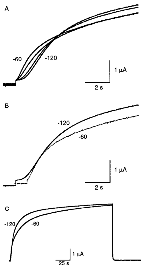
FIGURE 3 Effect of holding potential on activation of I_{SK} . (A) Currents elicited by step depolarization to 40 mV from holding potentials between -60 and -120 mV in 20-mV increments. (B) Comparison of currents elicited from a holding potential of -120 mV and -60 mV with the current trace recorded from a holding potential of -60 mV shifted by a delay of 0.91 s. (C) Long depolarization (3 min) to 40 mV from a holding potential of -120 and -60 mV.
